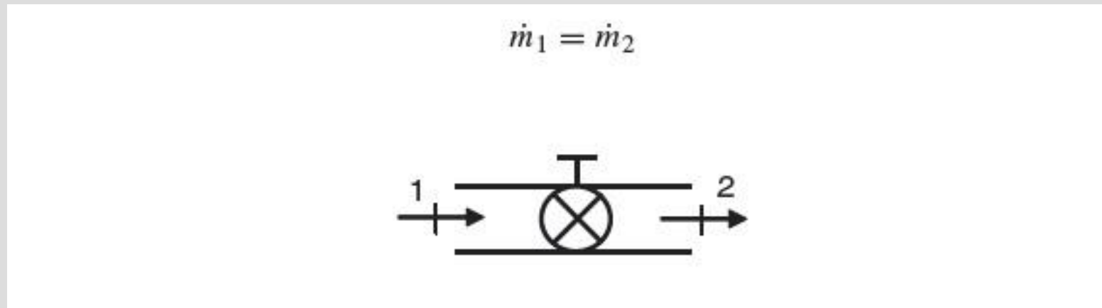
Figure 3.27 The schematic of a throttling valve considered for mass and energy analysis.
