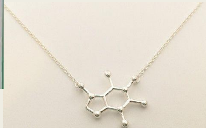
Caffeine Molecular Necklace
